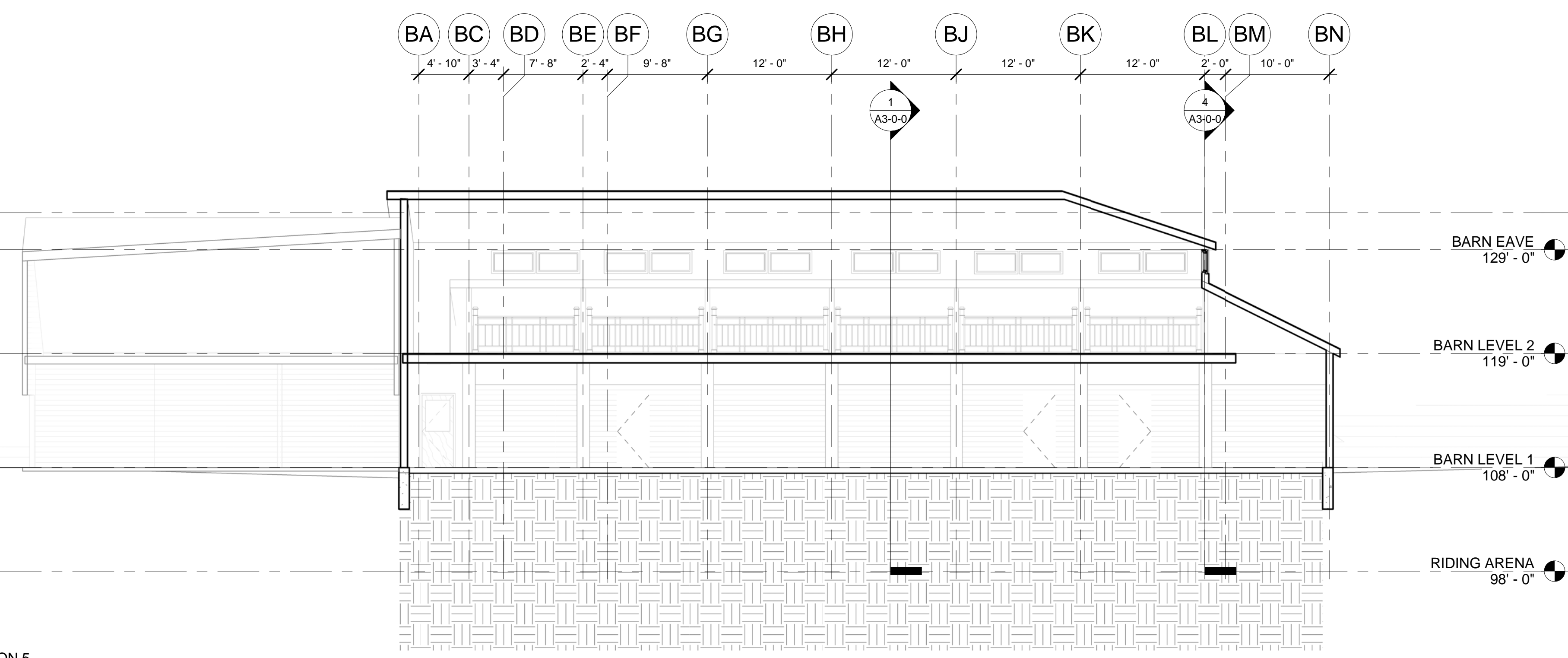
4 BUILDING SECTION 4 1/8" = 1'-0"
