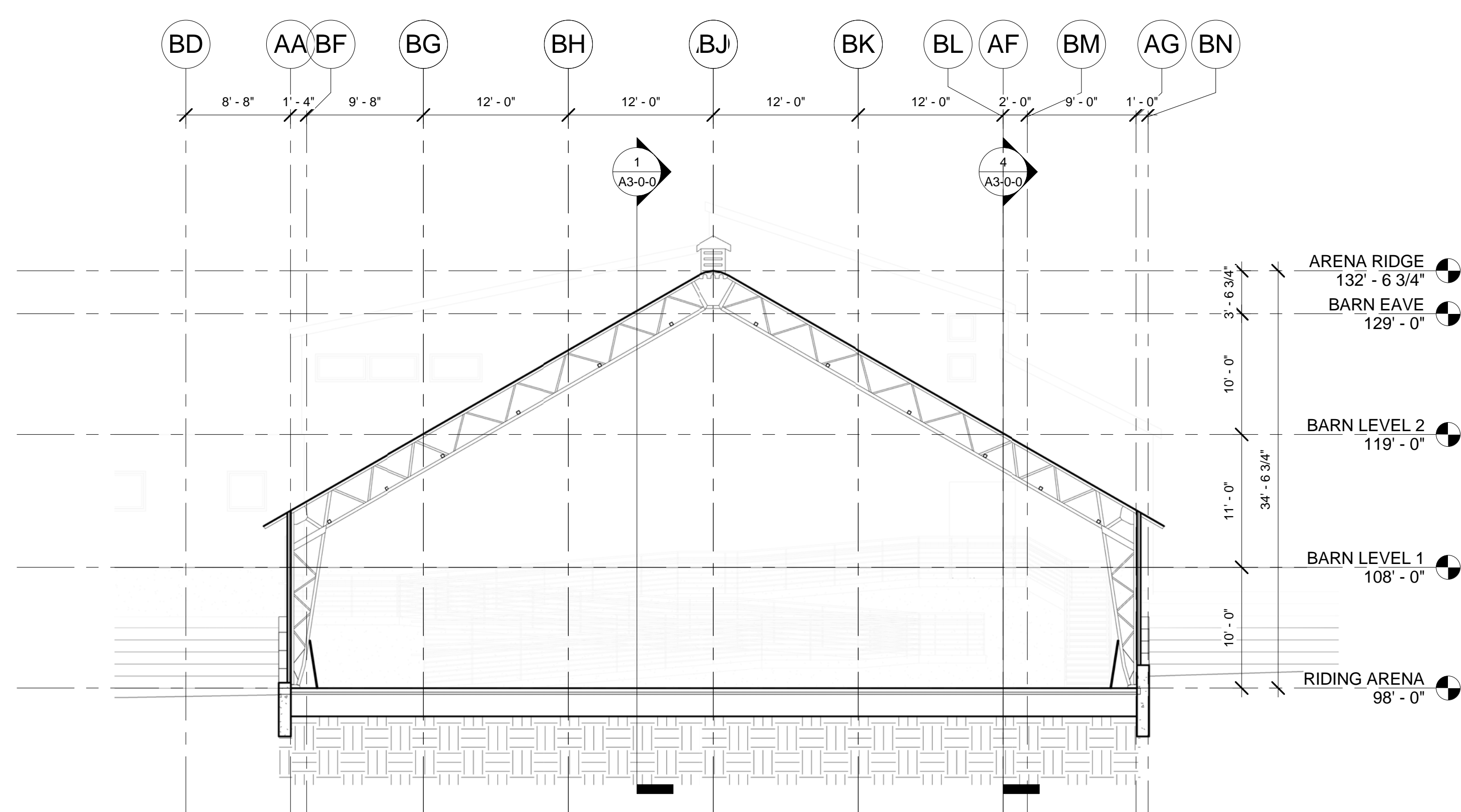
2 BUILDING SECTION 2 1/8" = 1'-0"
