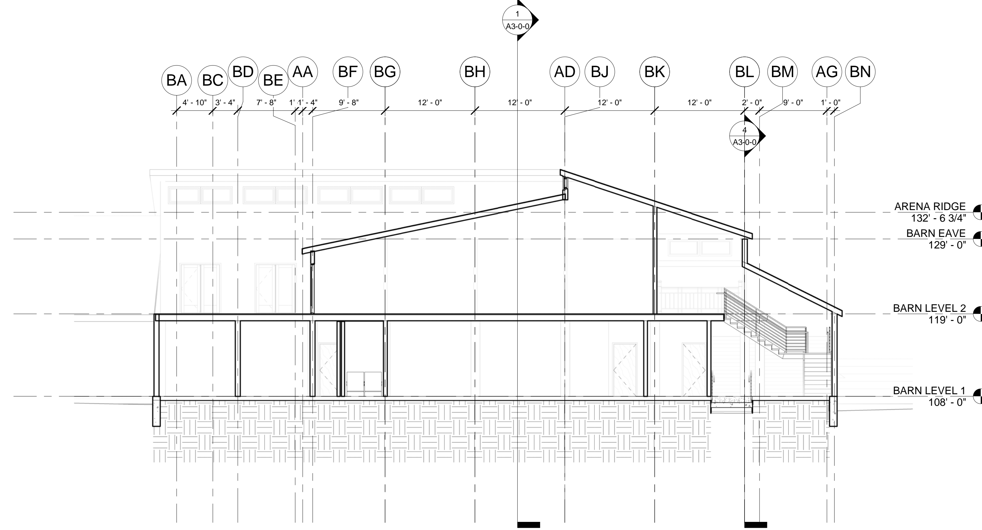
3 BUILDING SECTION 3 1/8" = 1'-0"
